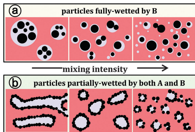
Fig. 4 Schematic of how mixing intensity affects structure when (a) particles are fully-wetted by phase B (shown in light blue), and (b) when particles are partially-wetted by both phases.
