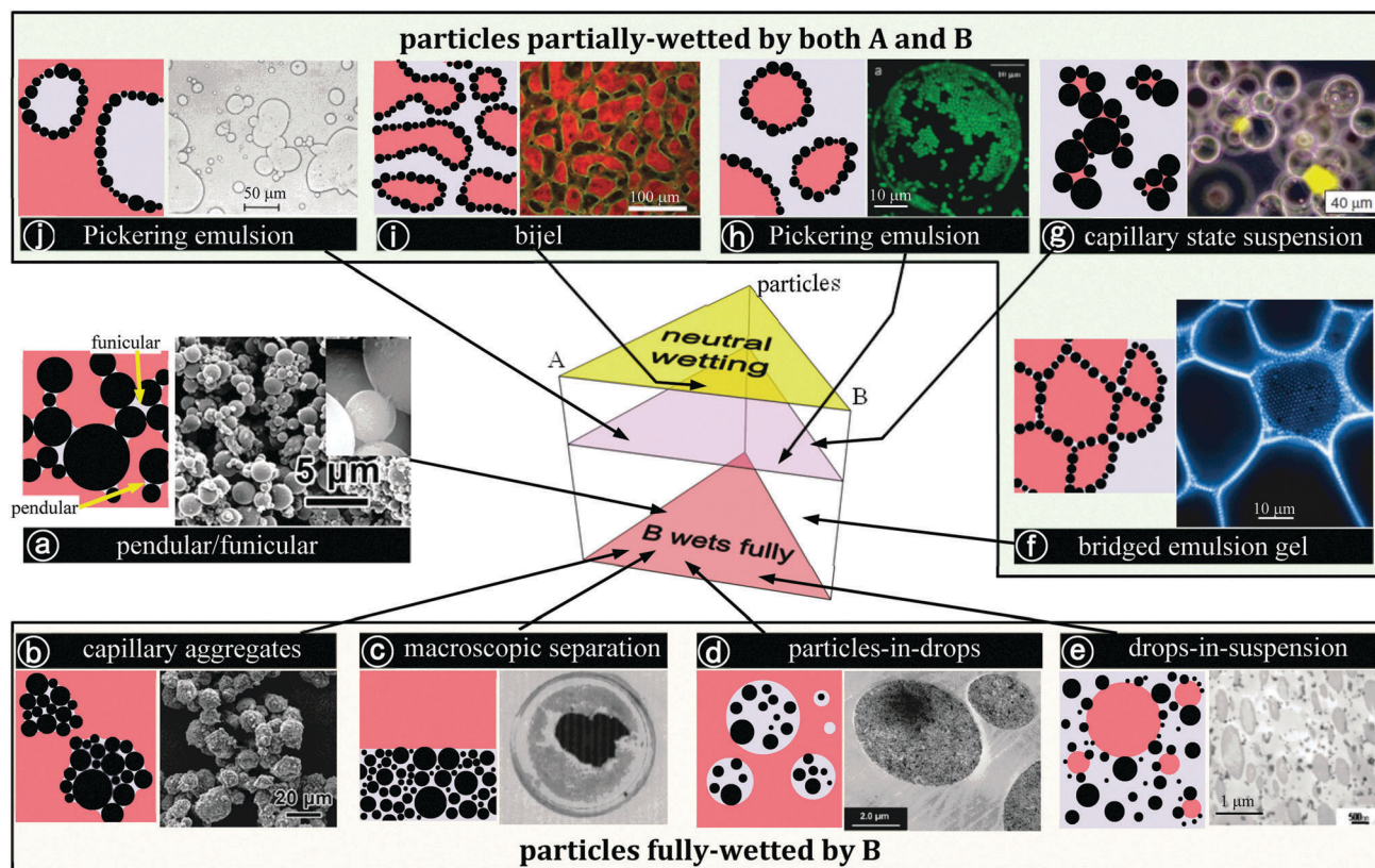
Fig. 2 Morphologies in various regions of the state prism for liquid/liquid/particle mixtures. Note that the prism does not extend up to full wettability by A, i.e. only the lower portion of the prism in Fig. 1c is shown. (a) Pendular morphology, 12,27 (b) capillary aggregates, 12 (c) macroscopically-separated system, 30 (d) particles-in-drops morphology, 57 (e) drops and particles both suspended in a matrix, 58 (f) bridged Pickering emulsion gels, 38 (g) capillary state suspension, 21 (h) Pickering emulsion, 59 (i) bijel, 54 (j) Pickering emulsion. Structures (b–e) require that the particles be fully-wetted by fluid B (shaded in light blue). Structures (f–j) require that particles be partially-wetted by both phases. The pendular/funicular structure, (a) can appear at both full as well as partial wettability. All images are reproduced from the literature as follows. (a and b) Reproduced from Domenech and Velankar, Soft matter , 2015, 11 , 1500 12 with permission from The Royal Society of Chemistry. (c) Reproduced from Sirianni et al. , Can. J. Chem. Eng. , 1969, 47 , 166 30 with permission from Wiley; all rights reserved. (d) Reprinted from Cai et al. , Polymer , 2012, 53 , 259, 57 Copyright (2012), with permission from Elsevier. (e) Reproduced from Lee et al. , Macromol. Mater. Eng. , 2012, 297 , 95 58 with permission from Wiley; All rights reserved. (f) Reprinted with permission from Lee et al. , Langmuir , 2012, 28 , 3085, 38 Copyright (2011) American Chemical Society (g) From Koos and N. Willenbacher, Science , 2011, 331 , 897. 21 Reprinted with permission from AAAS (h) reprinted with permission from Tarimala and Dai, Langmuir , 2004, 20 , 3492, 59 Copyright (2004) American Chemical Society. (i) Reproduced from Tavacoli et al. , Adv. Funct. Mater. , 2011, 21 , 2020 54 with permission from Wiley; All rights reserved. (j) Reprinted with permission from Binks and Lumsdon, Langmuir , 2000, 16 , 2539, 60 Copyright (2000) American Chemical Society.
