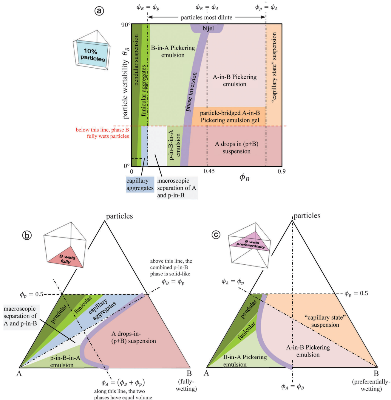
Fig. 3 State diagram represented in various cross sections (illustrated in the inset of each figure) of the triangular prism. Note that only the \theta range from 0° to 90° is shown, and hence fluid B fully or partially wets the particles. (a–c) Show three cross sections of the prism (a) at fixed particle volume fraction of \phi_p = 0.1 , (b) at fixed \theta near zero so that B fully wets the particles, and (c) at fixed \theta such that B wets the particles preferentially, but not fully. The various structures noted are illustrated schematically in Fig. 2.
