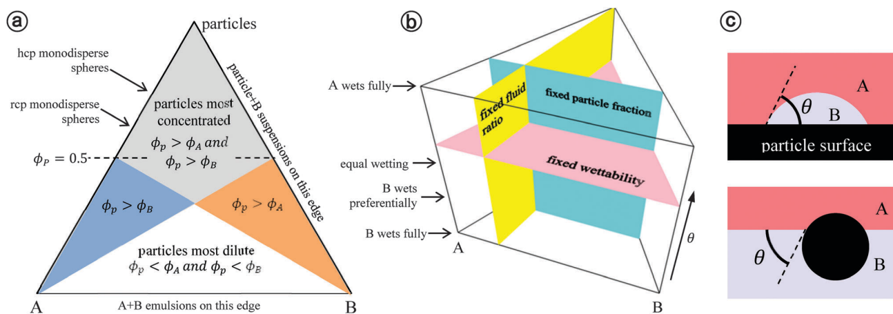
Fig. 1 (a) Schematic of ternary composition diagram marking various regions. (b) Ternary prism as particle wettability is changed. Various cross sections of the prism are labeled. (c) Two equivalent definitions of contact angle. Upper shows a drop on the surface of a solid surface with the contact angle measured through the B phase. Lower shows a spherical particle at the A/B interface making the same contact angle measured through the B phase.
