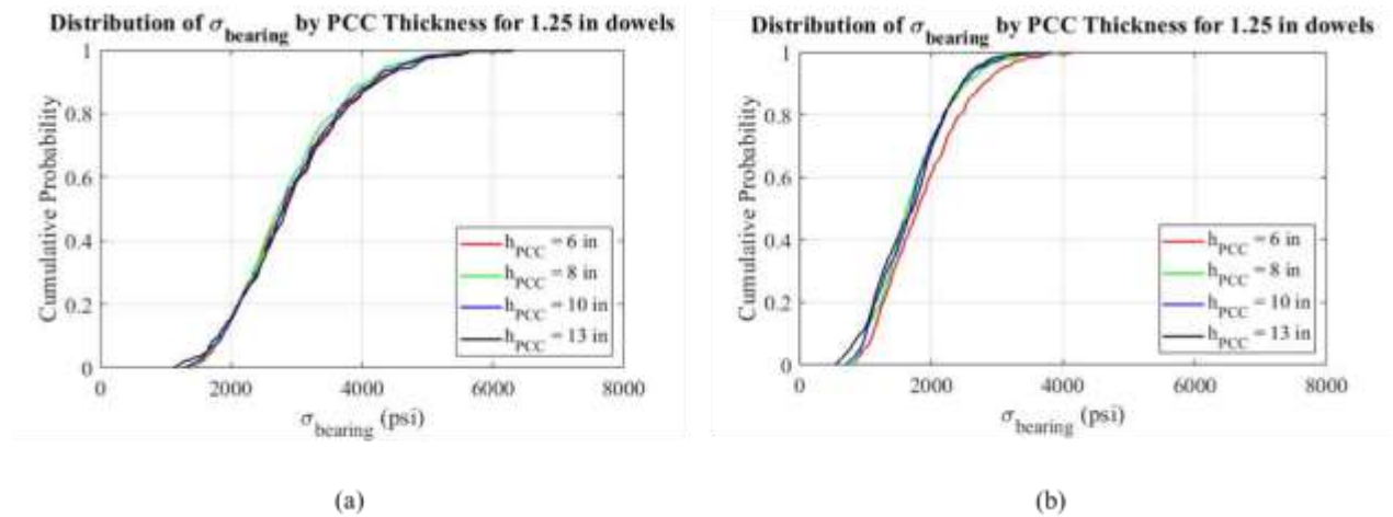
Figure 139: Cumulative distribution of bearing stress for a 1.25 in diameter dowel as a function of pavement thickness with (a) no aggregate interlock and (b) aggregate interlock (LTE=90%).
