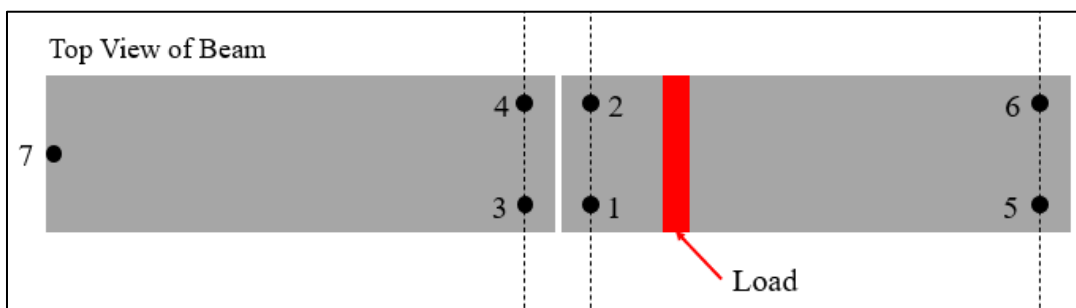
Figure 18: Plan view of beam test sensor layout.
