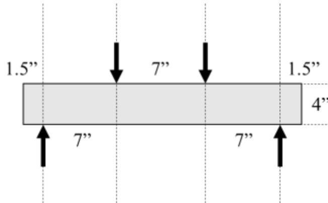
Figure 40: Four-point bending configuration used for 4-in x 4-in x 24-in concrete beam size.
