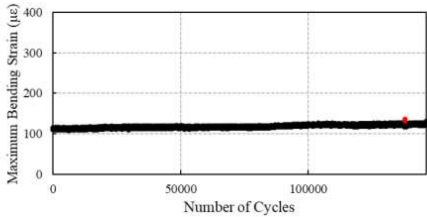
Figure 80: Maximum bending strain vs. number of cycles for (a) DCF_C4_B6 (overload of 0.8 at D = 15\% ) (b) DCF_C5_B7 (overload of 0.8 at D = 50\% ) and (c) DCF_C7_B3 (overload of 0.8 at D = 85\% ).
