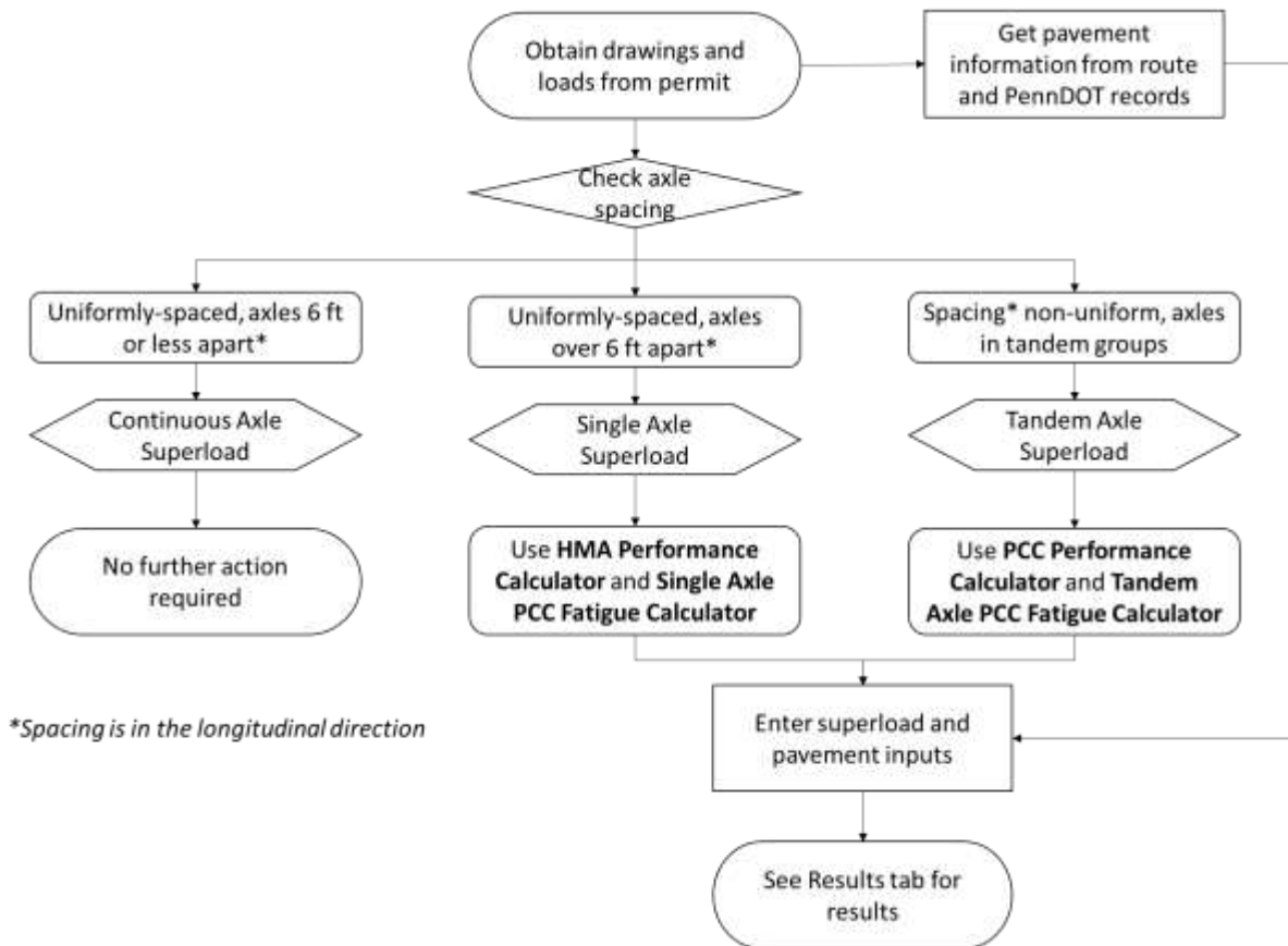
Figure 154: Flowchart for analyzing a SL with the provided tools
