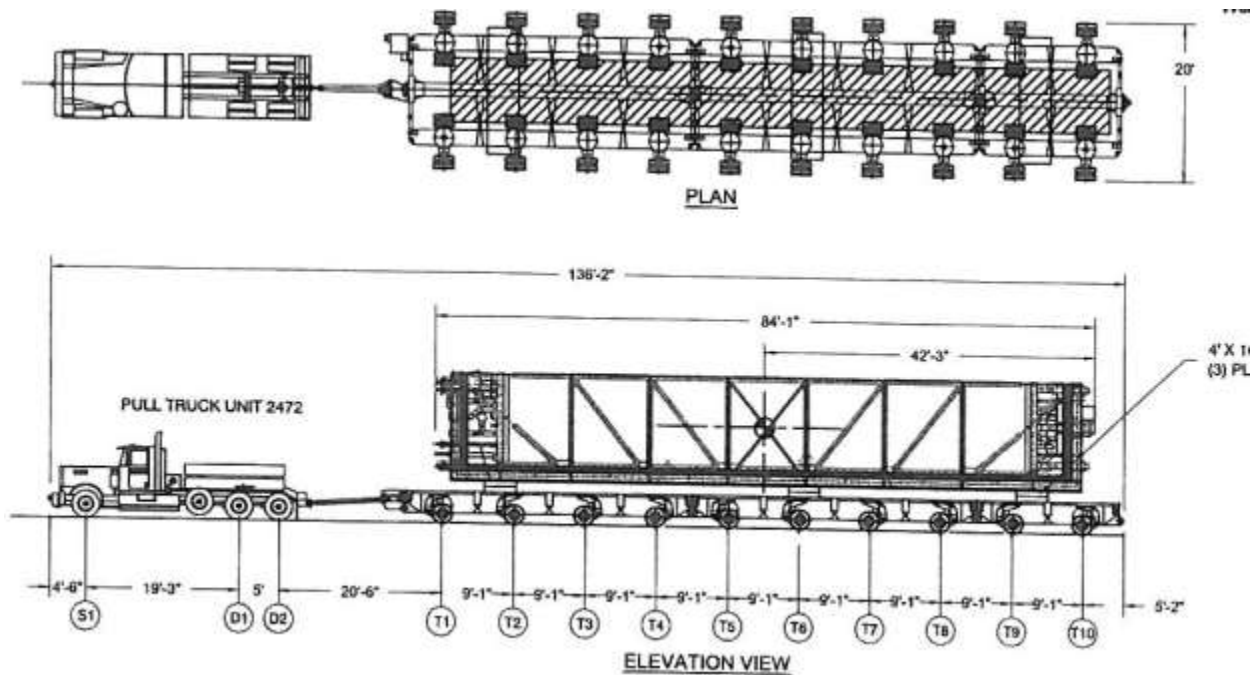
Figure 156: Plan and elevation view for Example 2
