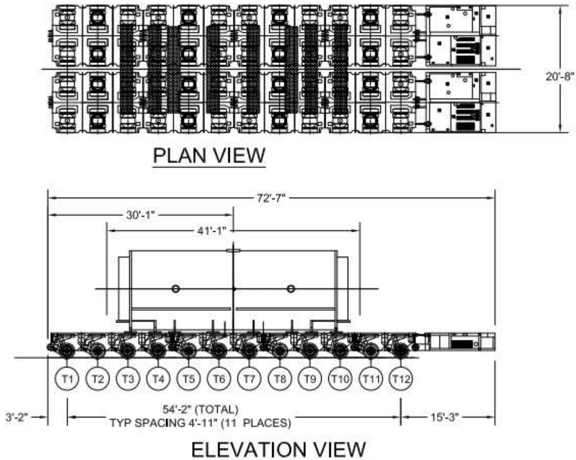
Figure 155: Plan and elevation view for Example 1
