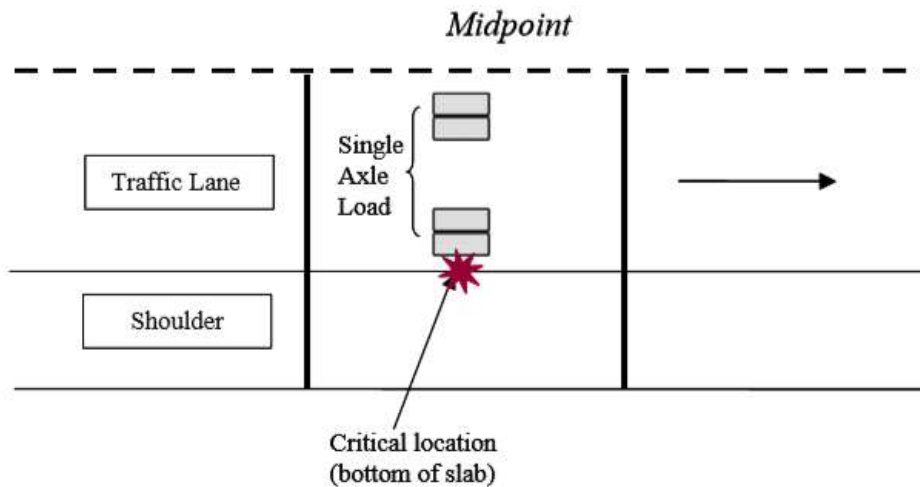
Figure 8: Critical loading position for the development of bottom-up cracking (Applied Research Associates (ARA), 2004).
