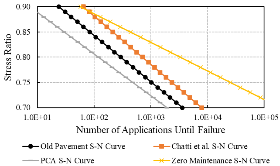
Figure 61: S-N curve comparisons for (a) new pavement strength and (b) old pavement strength.
